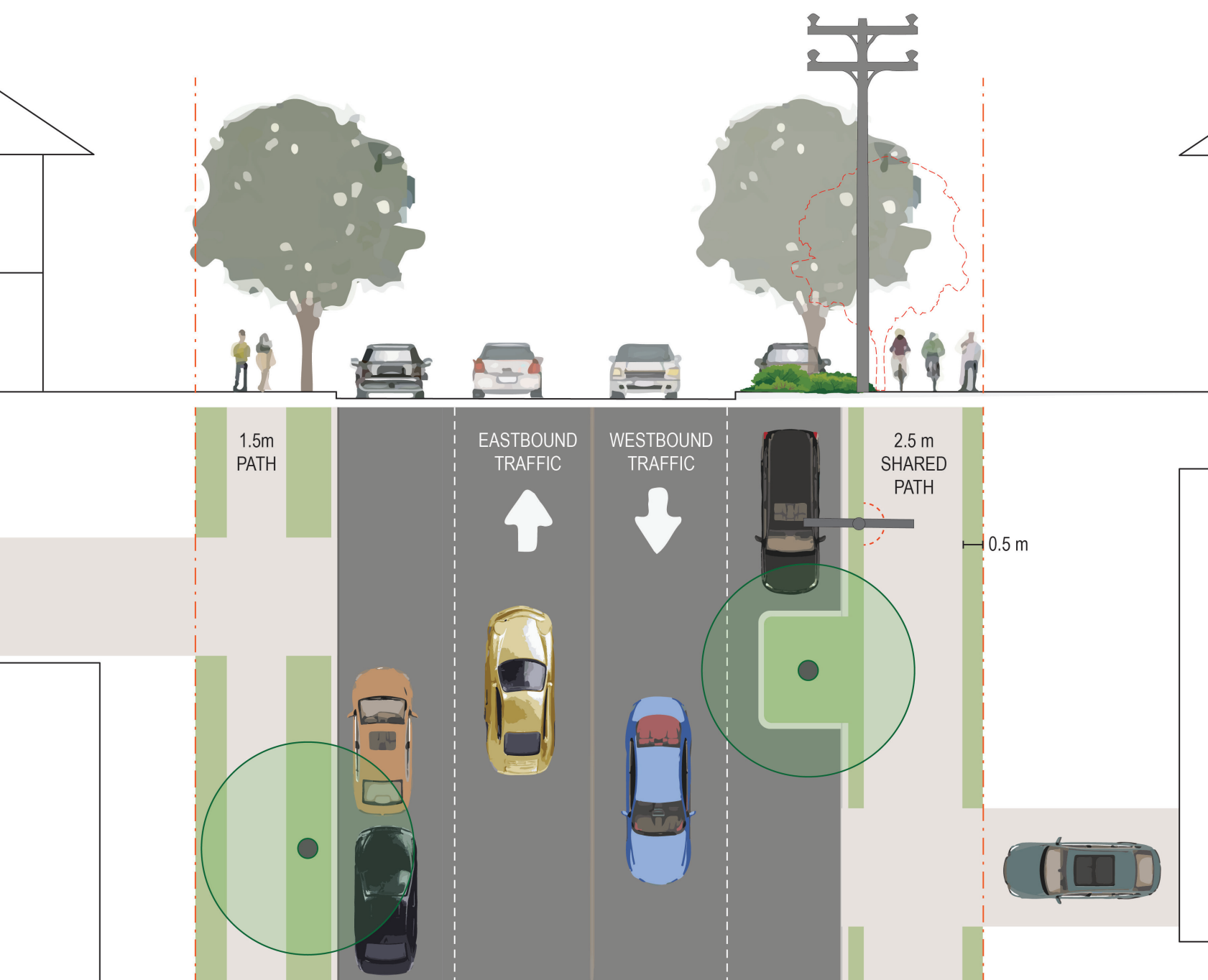
Diagram showing the typical street layout and upgraded footpath at Spring Street
